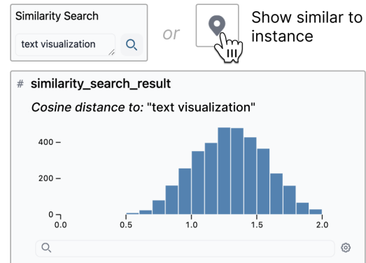
Figure 6.4: Document embeddings enable a projection overview and similarity search.
