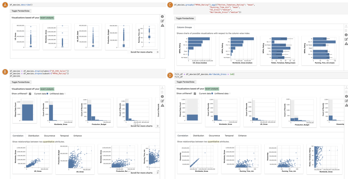
Figure 5.5: SOLAS tracks history throughout an analysis to provide improved visualizations. We show four snapshots from an example analysis that demonstrate the recommendations from SOLAS. (A) When an analyst calls describe , we visualize the returned data as a boxplot by using information that is no longer present in the returned data to plot outliers. (B) After cleaning their data by dropping columns and nulls, SOLAS shows how the distribution of other columns change. (C) For groupbys and aggregations, we use history information to add better x-axis labels and include error bars when plotting the mean. (D) When filtering, SOLAS shows the background distribution of each column from the parent data relative to the filtered data. Users can toggle the background distribution on and off.
