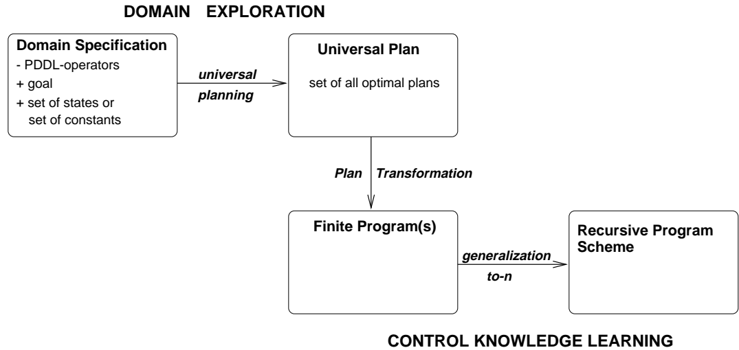
Figure 4.1: Induction of Recursive Functions from Plans
