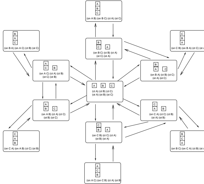
Figure 3.2: Problem Graph for the Tower Problem
