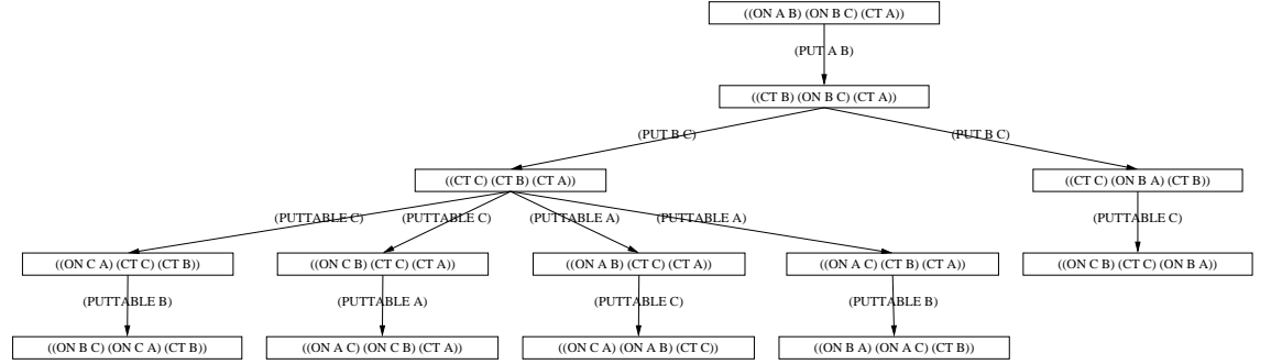
Figure 4.20: Plan for Tower with Three Blocks
