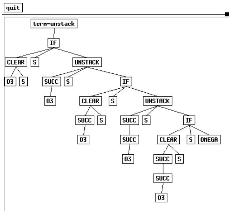
Figure 4.8: Finite Program for the Unstack Domain
