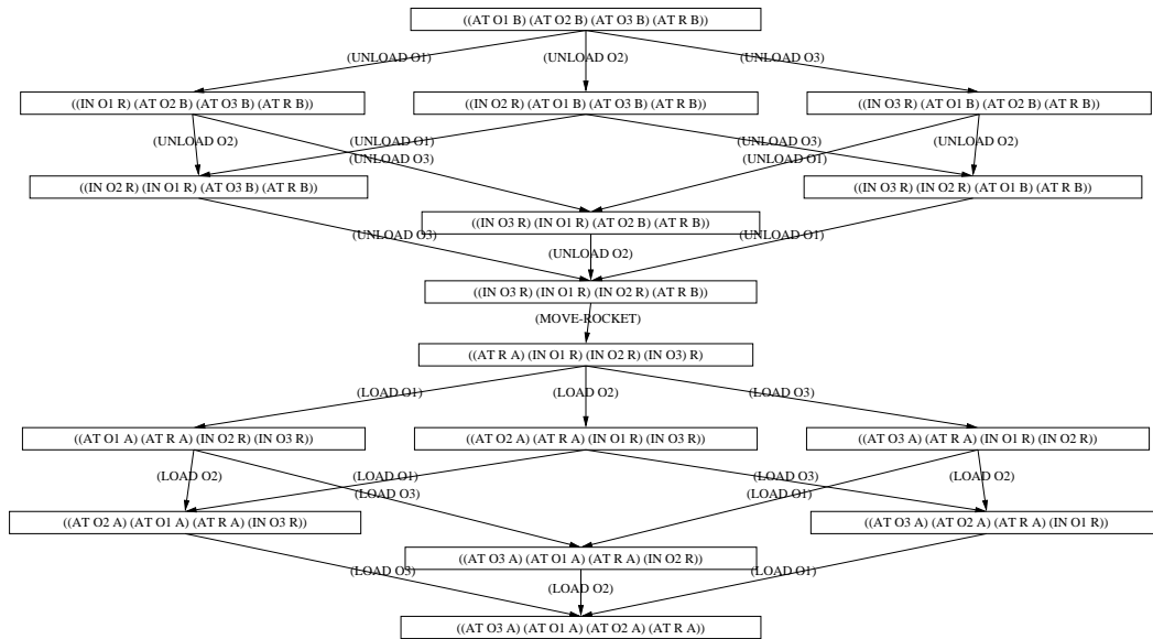
Figure 2.1: Optimal Universal Plan for Rocket ( in = inside , R = rocket )
