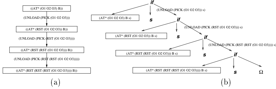
Figure 2.3: Introduction of the Data Type Set (a) and Resulting Finite Program (b) for the Unload-All Sub-Plan of Rocket ( \Omega denotes “undefined”)
